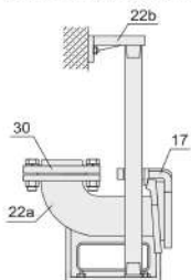
Auto-coupled Installation(Z)
